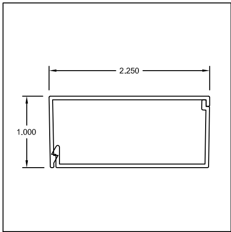
Part #: US031 / US032 Name: 1" x 2-1/4" Trim & Clip
