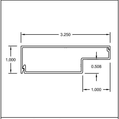
Part #: US121 / US138 Name: 1" x 3-1/4" Trim & Z-Clip
