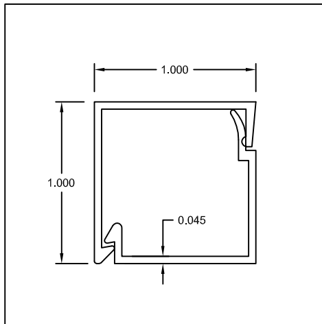
Part #: US010 / US016 Name: 1" x 1" Trim & Clip
