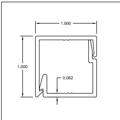
Part #: CES088 / CES089 Name: 1" x 1" Trim & Clip
