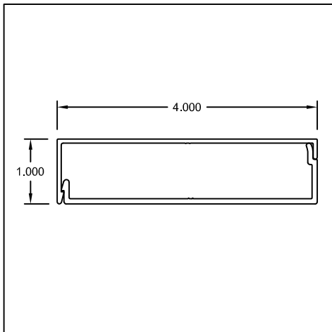
Part #: US157 / US158 Name: 1" x 4" Trim & Clip
