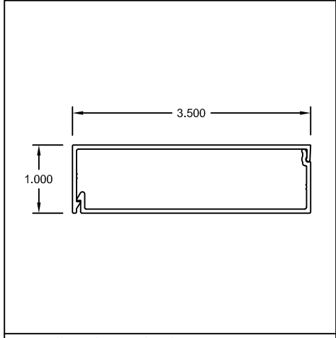
Part #: US286 / US287 Name: 1" x 3-1/2" Trim & Clip
