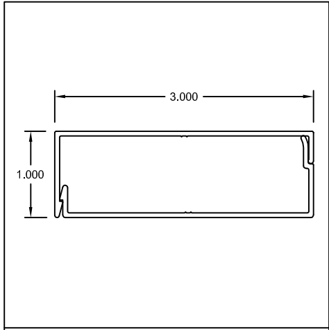
Part #: US151 / US152 Name: 1" x 3" Trim & Clip
