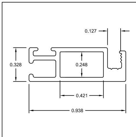
Part #: CES062 Name: Screen Frame
