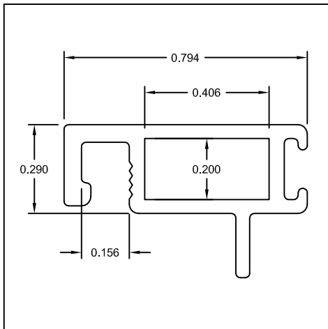
Part #: US002 Name: Screen Frame w/ 0.210" Leg
