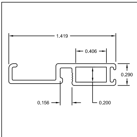
Part #: US004 Name: Screen Frame w/ Handle
