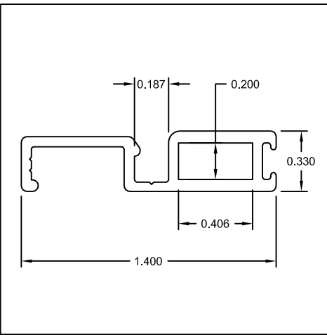
Part #: U6034 Name: Screen Frame
