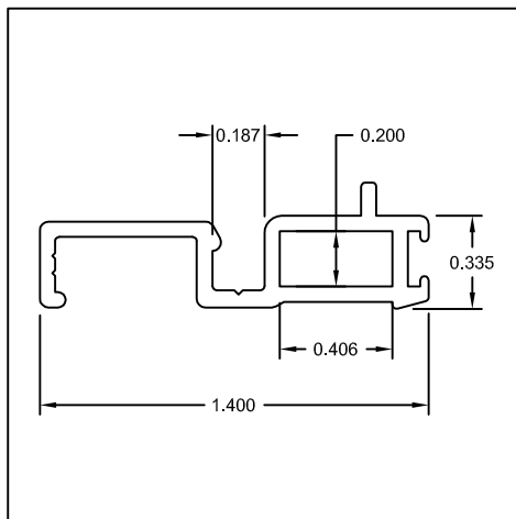
Part #: US050 Name: Screen Frame w/ 0.120" Leg
