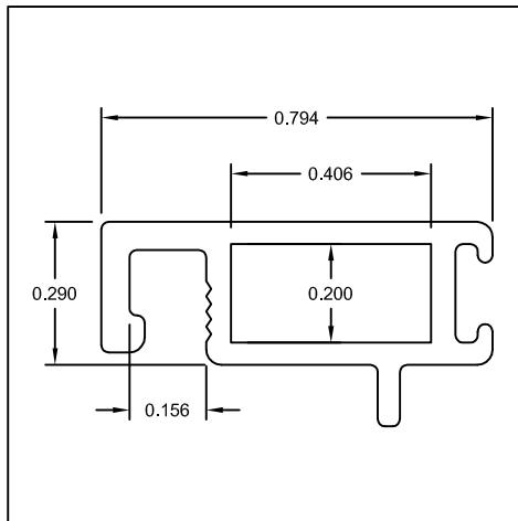
Part #: US003 Name: Screen Frame w/ 0.125" Leg
