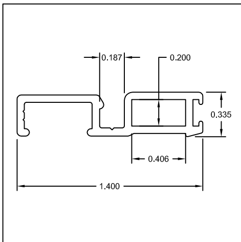
Part #: US051 Name: Screen Frame
