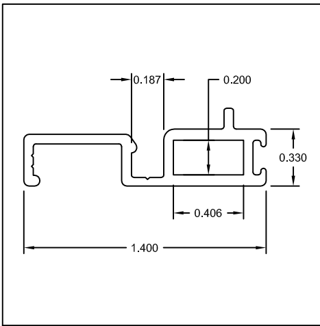
Part #: U6035 Name: Screen Frame w/ 0.120" Leg
