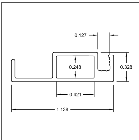
Part #: CES061 Name: Screen Frame w/ Handle
