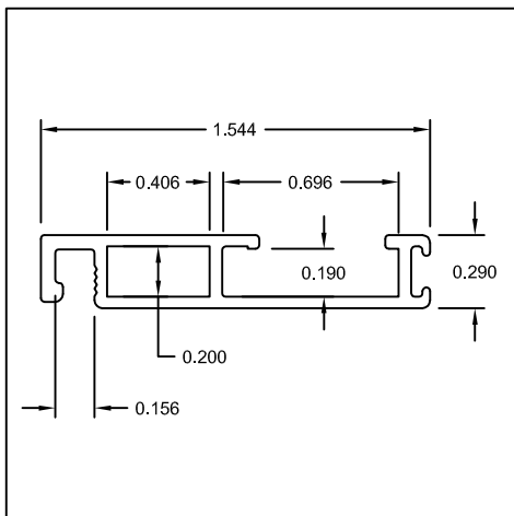
Part #: US005 Name: Screen Frame w/ Lock
