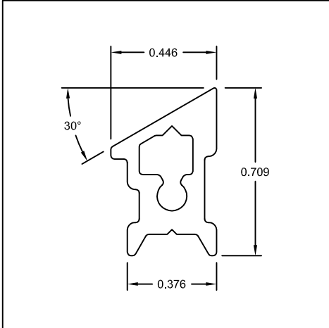
Part #: US129 Name: 3/8" X 3/4" Muntin Frame
