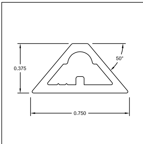
Part #: US118 Name: 3/8" X 3/4" Muntin Grid
