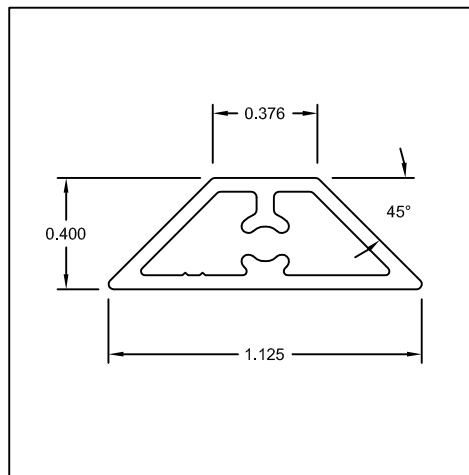
Part #: CES082 Name: 3/8" X 1-1/8" Muntin Grid
