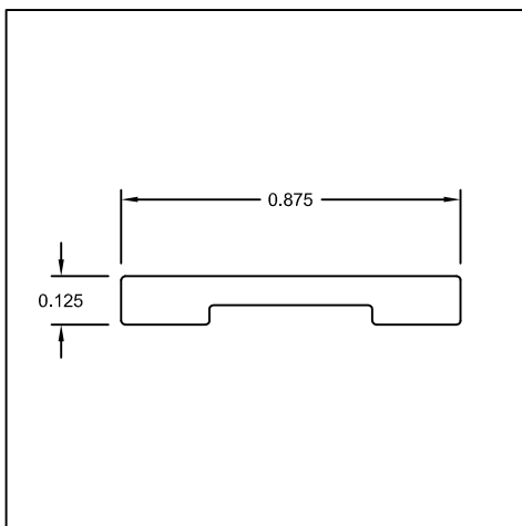
Part #: US028 Name: 1/8" X 7/8" Muntin Grid
