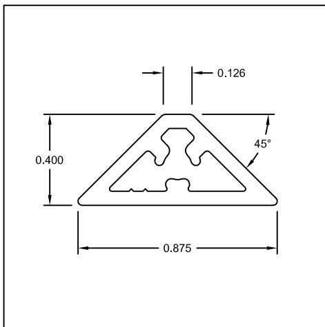
Part #: CES081 Name: 3/8" X 7/8" Muntin Grid
