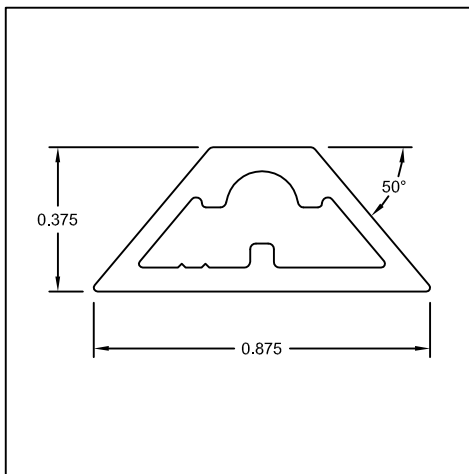
Part #: US239 Name: 3/8" X 7/8" Muntin Grid
