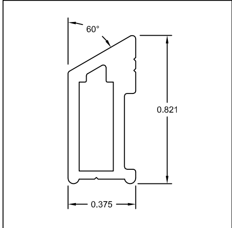
Part #: US183 Name: 3/8" X 7/8" Muntin Frame
