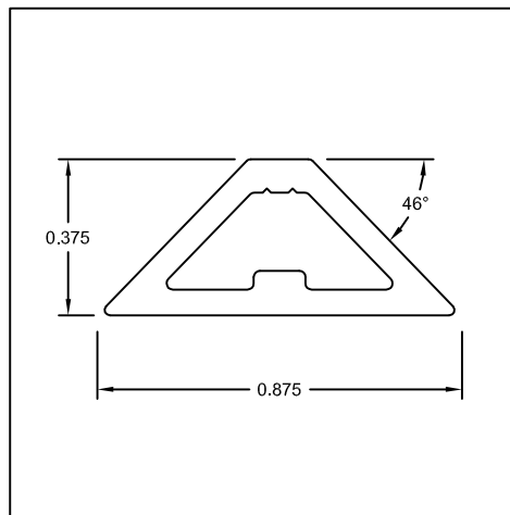
Part #: US026 Name: 3/8" X 7/8" Muntin Grid
